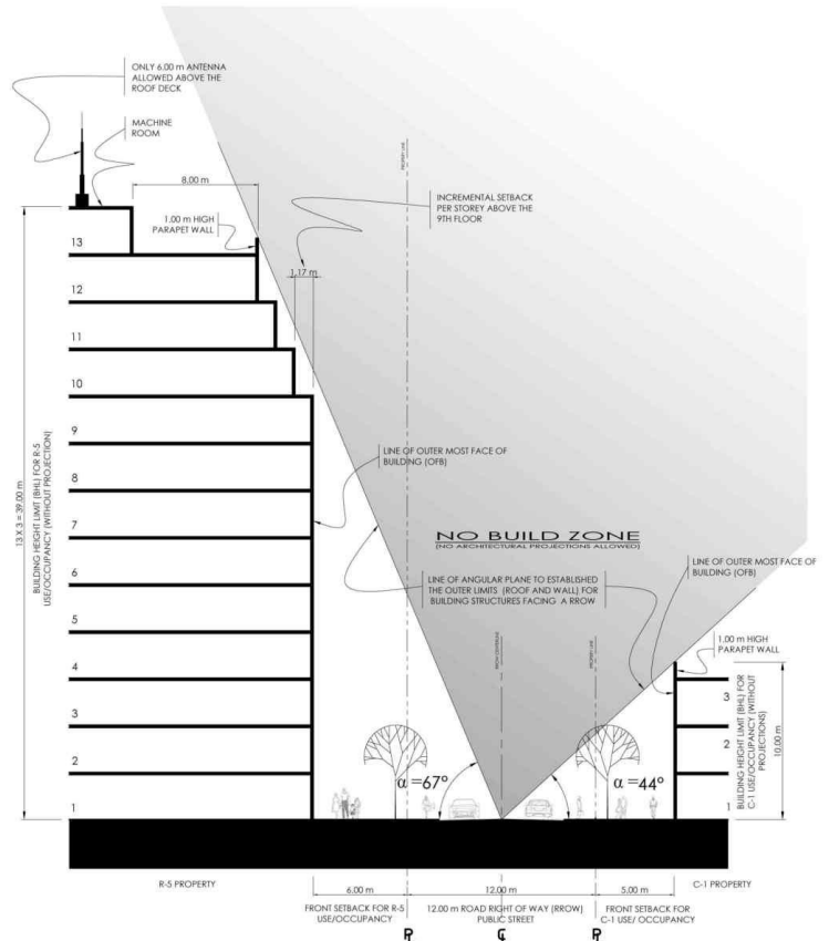
ROW ANGLES FROM CENTERLINE THAT DETERMINE THE OFB OF BUILDINGS/STRUCTURES ALONG A 12.00 m ROW
