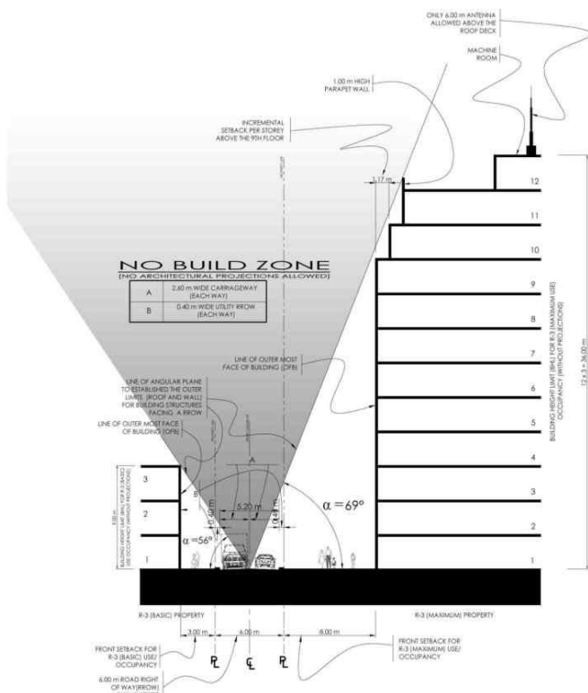
ROW ANGLES FROM CENTERLINE THAT DETERMINE THE OFB OF BUILDINGS/STRUCTURES ALONG A 6.00 m ROW
