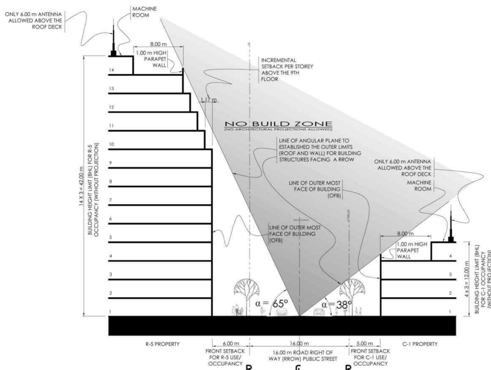
ROW ANGLES FROM CENTERLINE THAT DETERMINE THE OFB OF BUILDINGS/STRUCTURES ALONG A 16.00 m ROW
