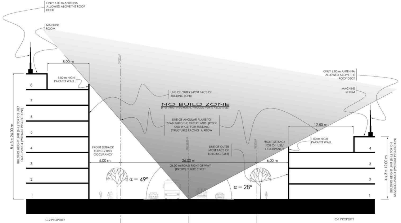
RROW ANGLES FROM CENTERLINE THAT DETERMINE THE OFB OF BUILDINGS/STRUCTURES ALONG A 26.00 m RROW
