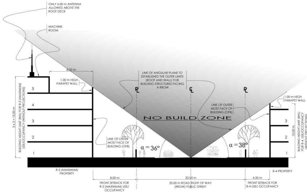
ANGLES FROM CENTERLINE THAT DETERMINES THE OFB OF BUILDINGS/STRUCTURES ALONG A 20.00 m RROW
