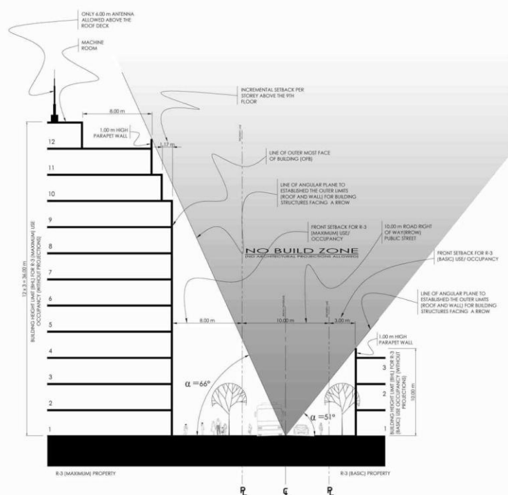
ANGLES FROM CENTERLINE THAT DETERMINE THE OFB OF BUILDINGS/STRUCTURES ALONG A 10.00 m ROW
