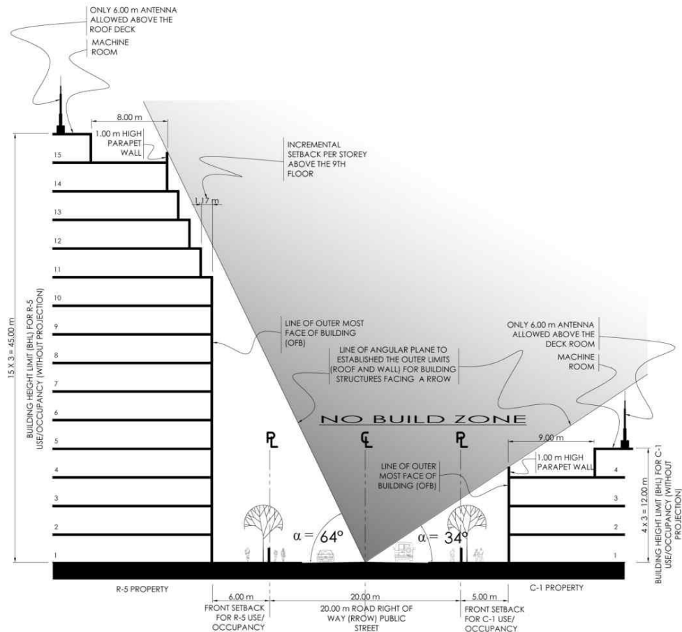
ANGLES FROM CENTERLINE THAT DETERMINES THE OFB OF BUILDINGS/STRUCTURES ALONG A 20.00 m RROW
