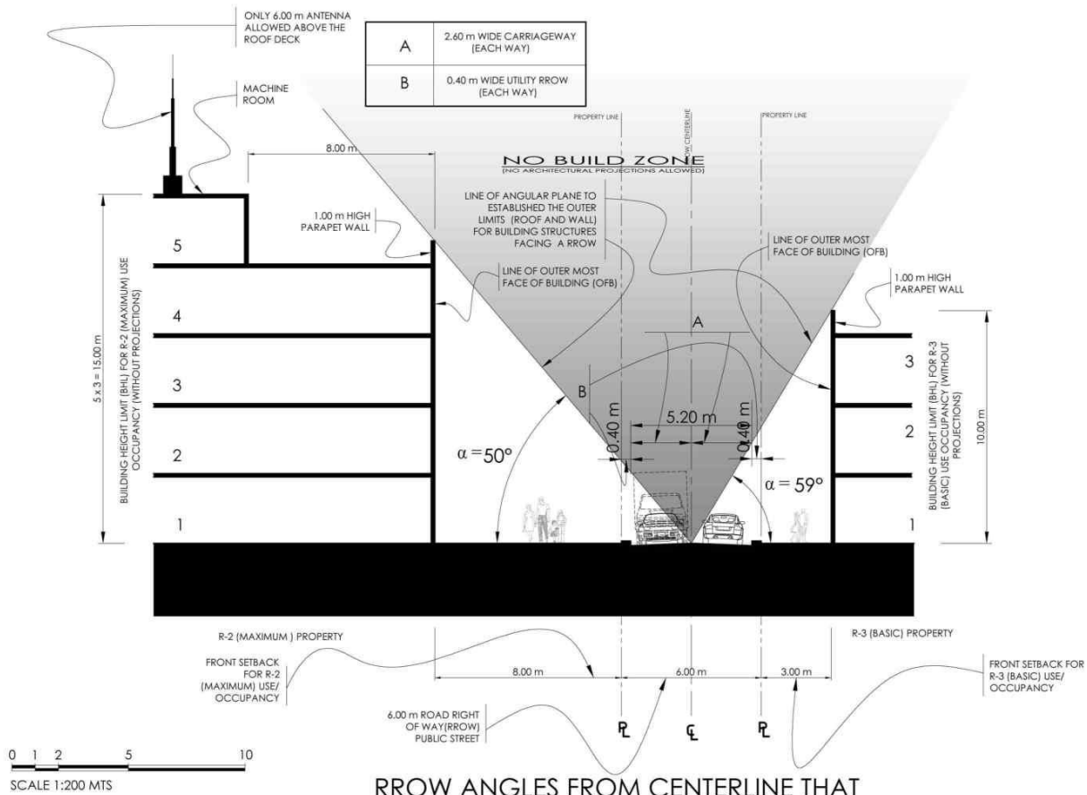
ROW ANGLES FROM CENTERLINE THAT DETERMINE THE OFB OF BUILDINGS/STRUCTURES ALONG A 6.00 m
